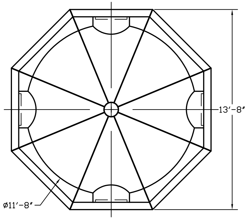
DM058 - 8 PIECE DOME WITH OPENINGS FOR WINDOWS
