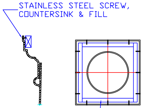
BLOCKING AS REQUIRED BLOCKING DETAIL, CAPITAL
