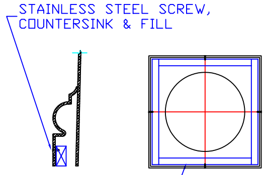
BLOCKING AS REQUIRED BLOCKING DETAIL, BASE
